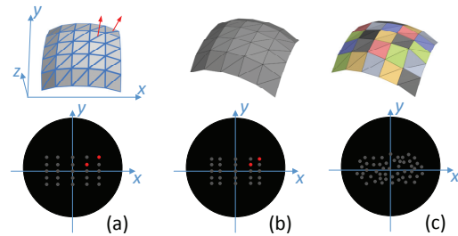
Figure 4: Initialization. (a) By assuming each height field quad lies in the same plane and the patch shape is symmetric and convex, the facet normals form an axis-aligned grid in the angular domain and thus is determined by two normals (marked in red) for a 6 \times 6 height field. (b) The initial height field for a bi-scale material patch. (c) The optimized height field of the bi-scale material patch.
