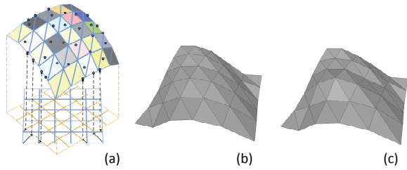
Figure 5: Shading frame mapping. (a) The bi-scale material patch obtained in the last step is rotated back to its shading frame and resampled by the regular grid of the height field (shown in blue). (b) The resampled height field patch. (c) The height field patch after optimization.
